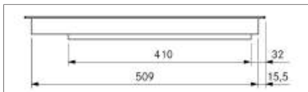
Fig. 3.10 PKI3 appliance dimensions side view
