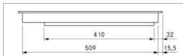
Fig. 3.13 PKI3 appliance dimensions side view
