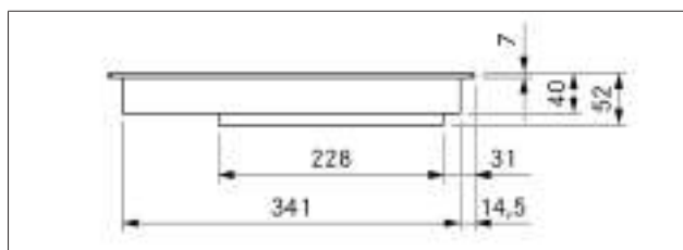
Fig. 3.9 PKI3 appliance dimensions front view
